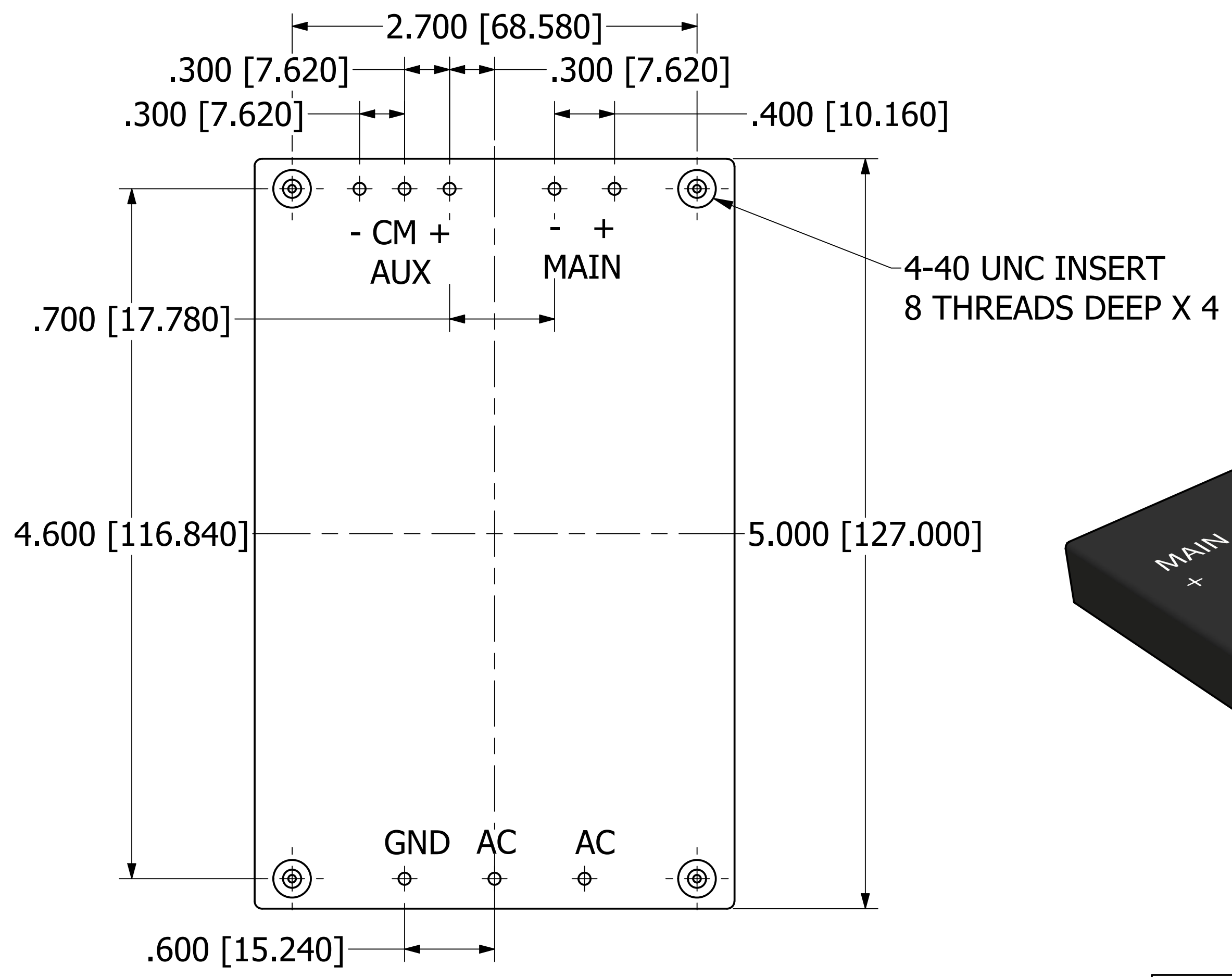
BOTTOM VIEW
